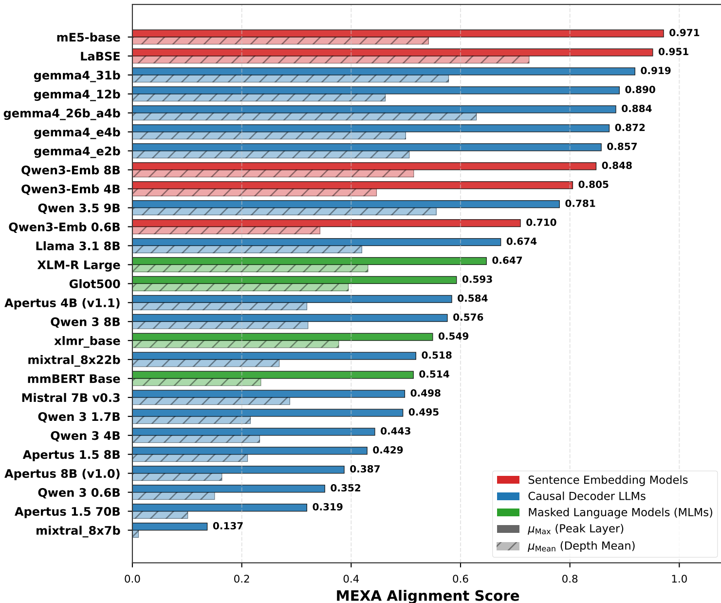
Cross-Lingual Representation Alignment Scores on FLORES (All Models)
